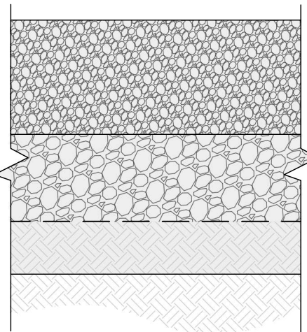
ACCESS ROAD RECONSTRUCTION GRAVEL STRUCTURE
