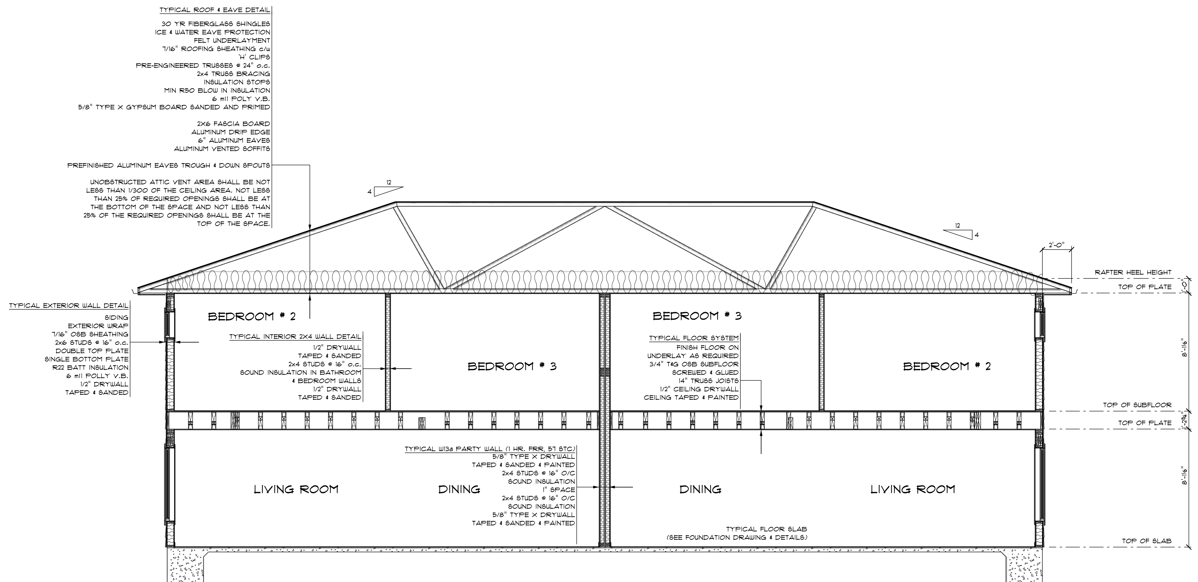
CROSS SECTION A SCALE: 1/4" = 1'-0"
