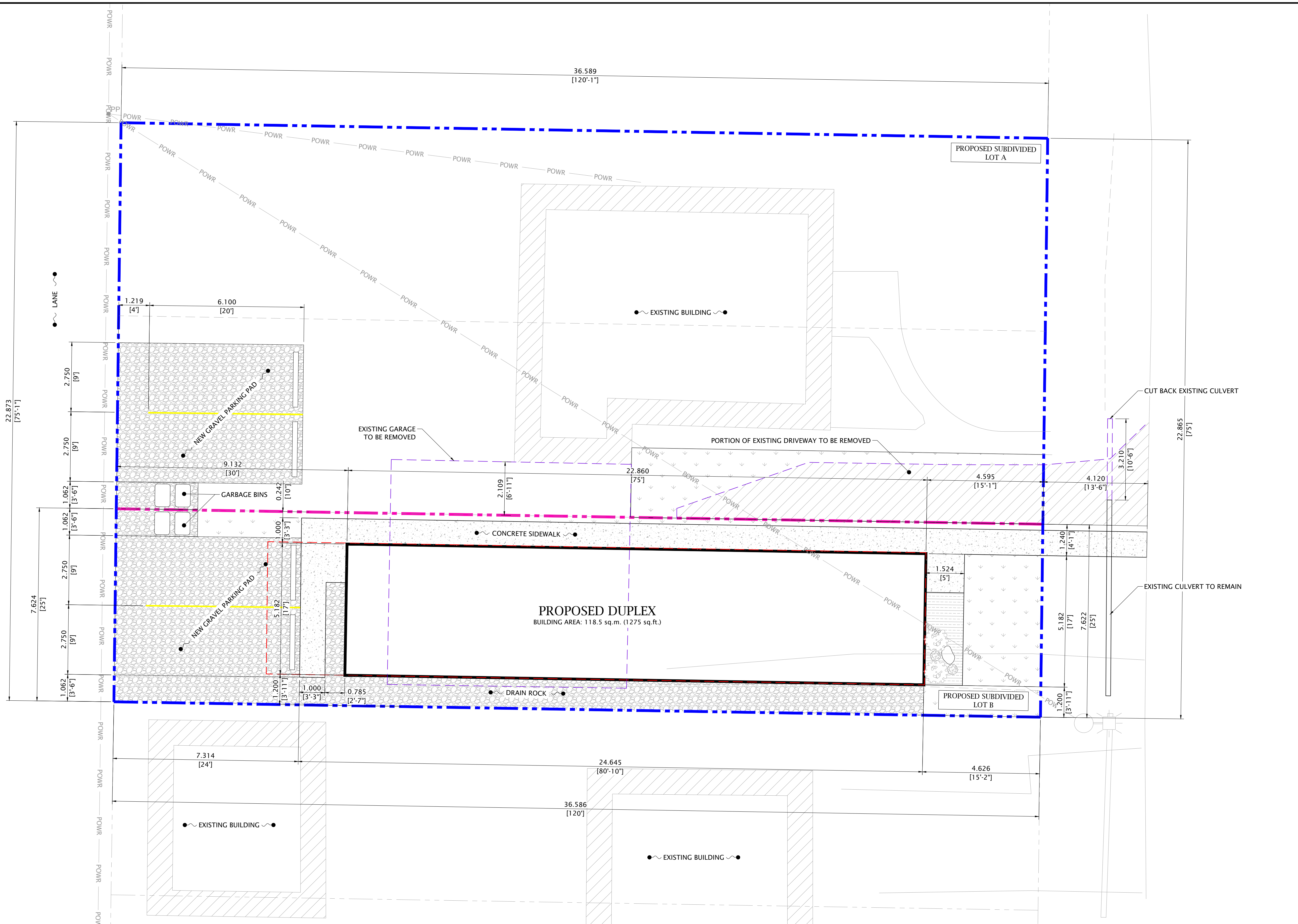
1 SITE CONCEPT PLAN SCALE: 1:75
