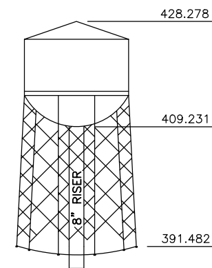
DETAIL - WATER TOWER BUILT- 1930. 625,000 Gal - 100,000 Cu Ft [NOT IN USE]
